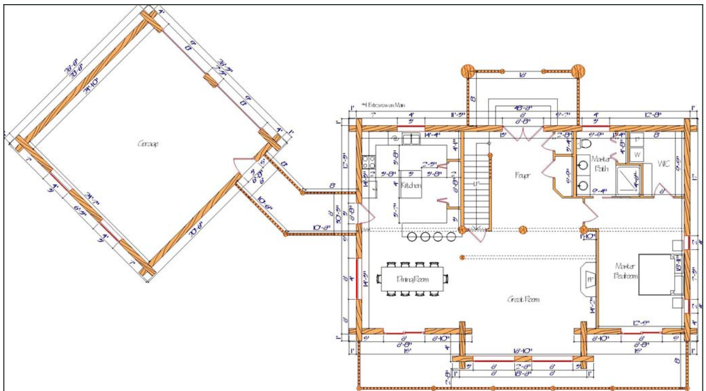
Floor Plan — View 1
