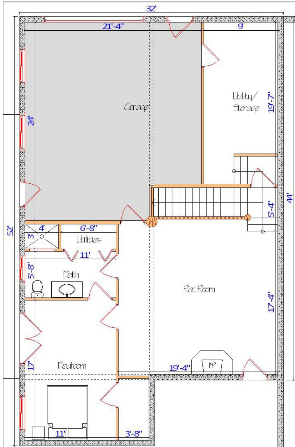
Floor Plan — View 3
