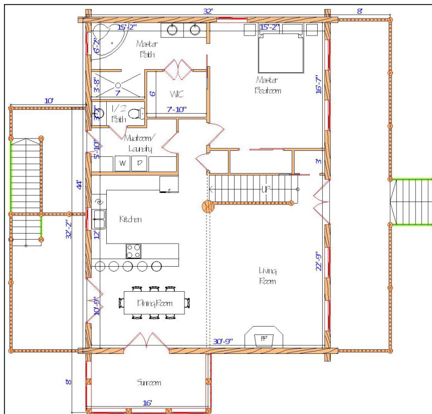
Floor Plan — View 1
