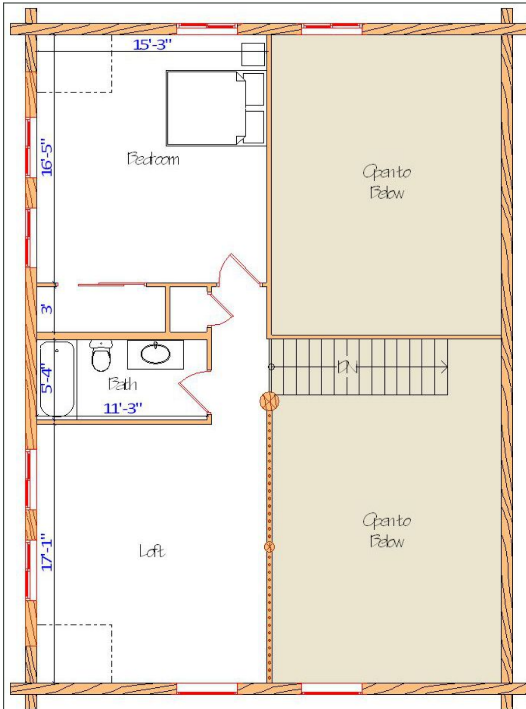
Floor Plan — View 2
