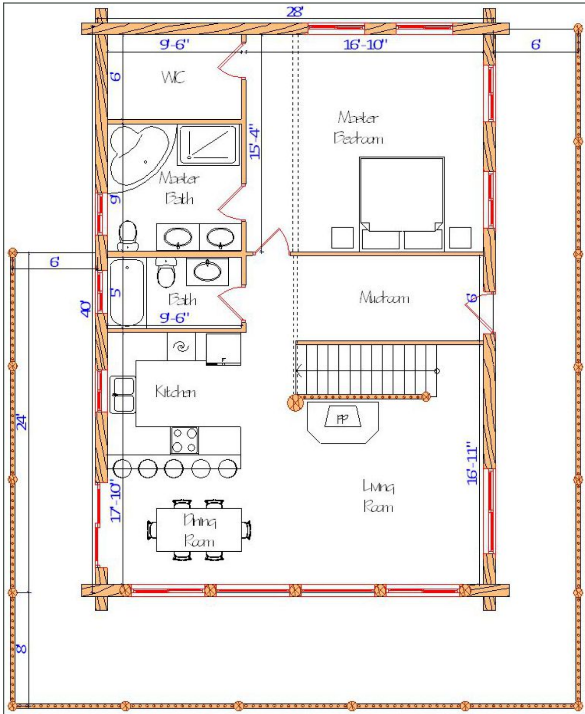
Floor Plan — View 2
