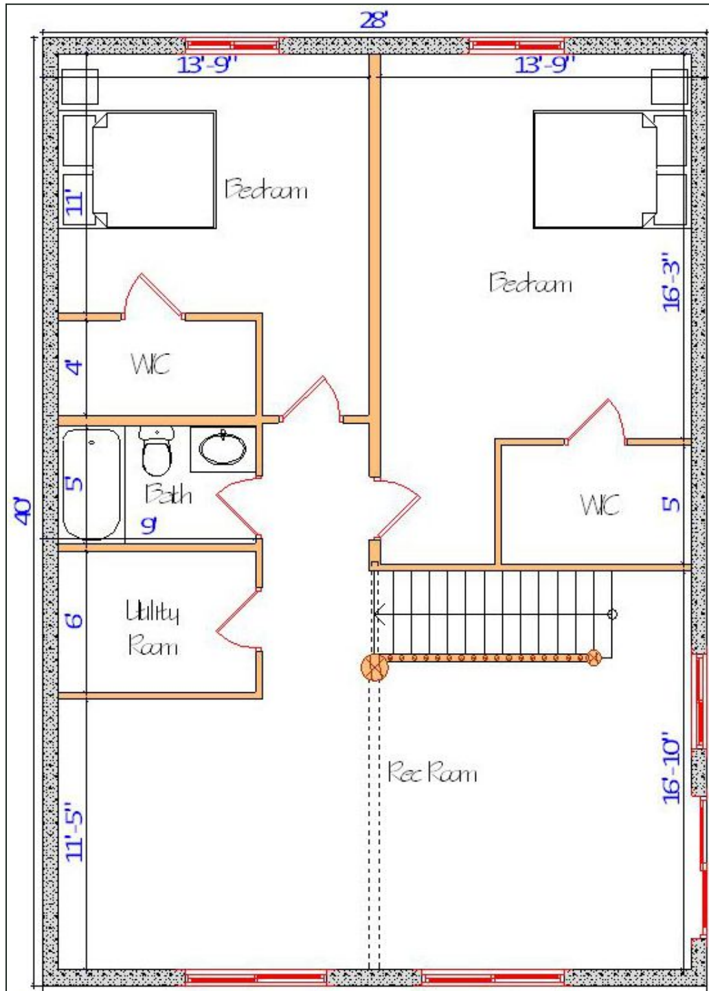
Floor Plan — View 3
