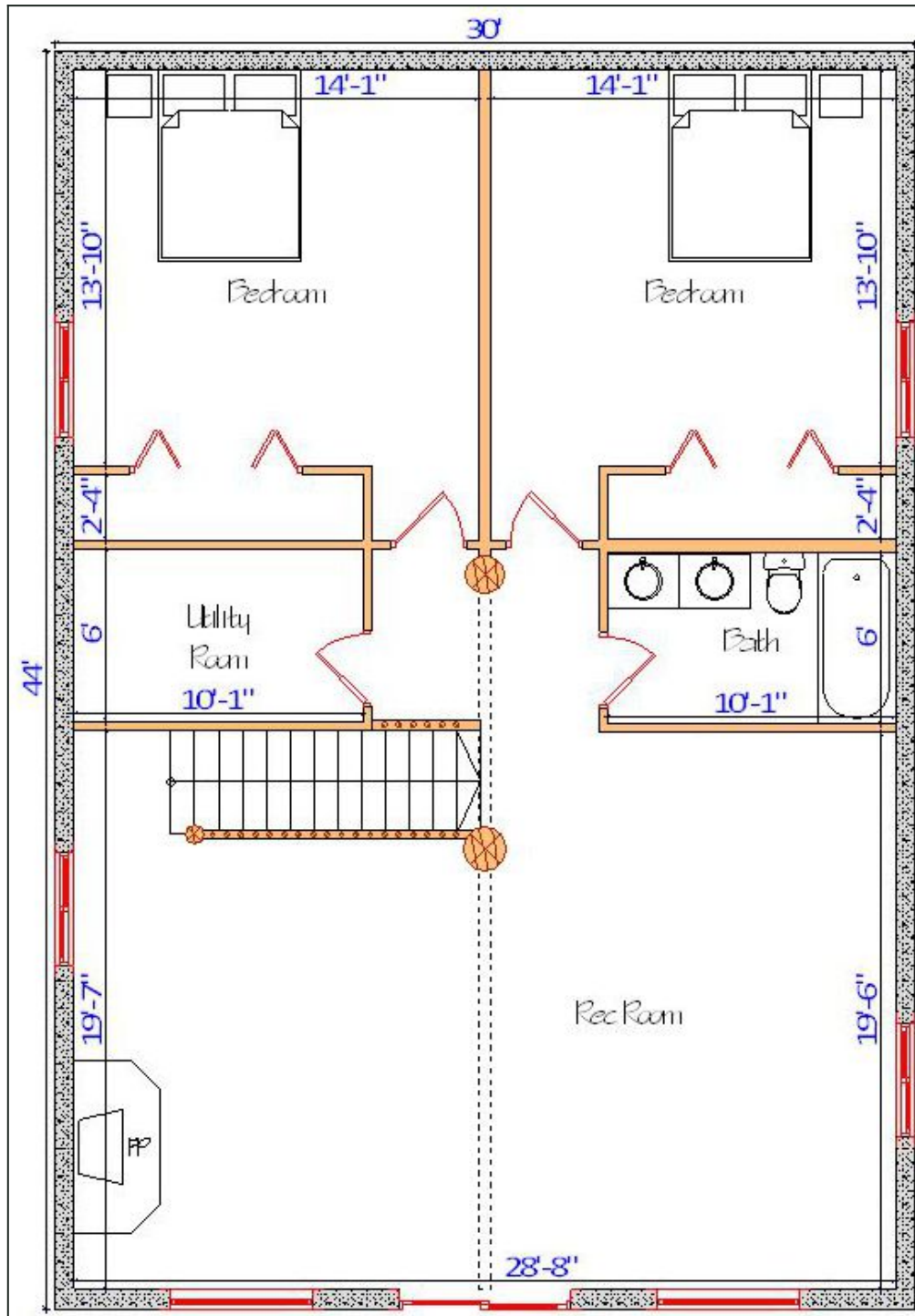
Floor Plan — View 3
