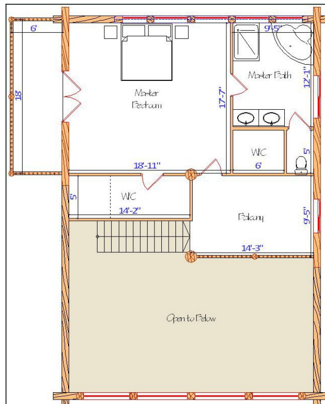
Floor Plan — View 1
