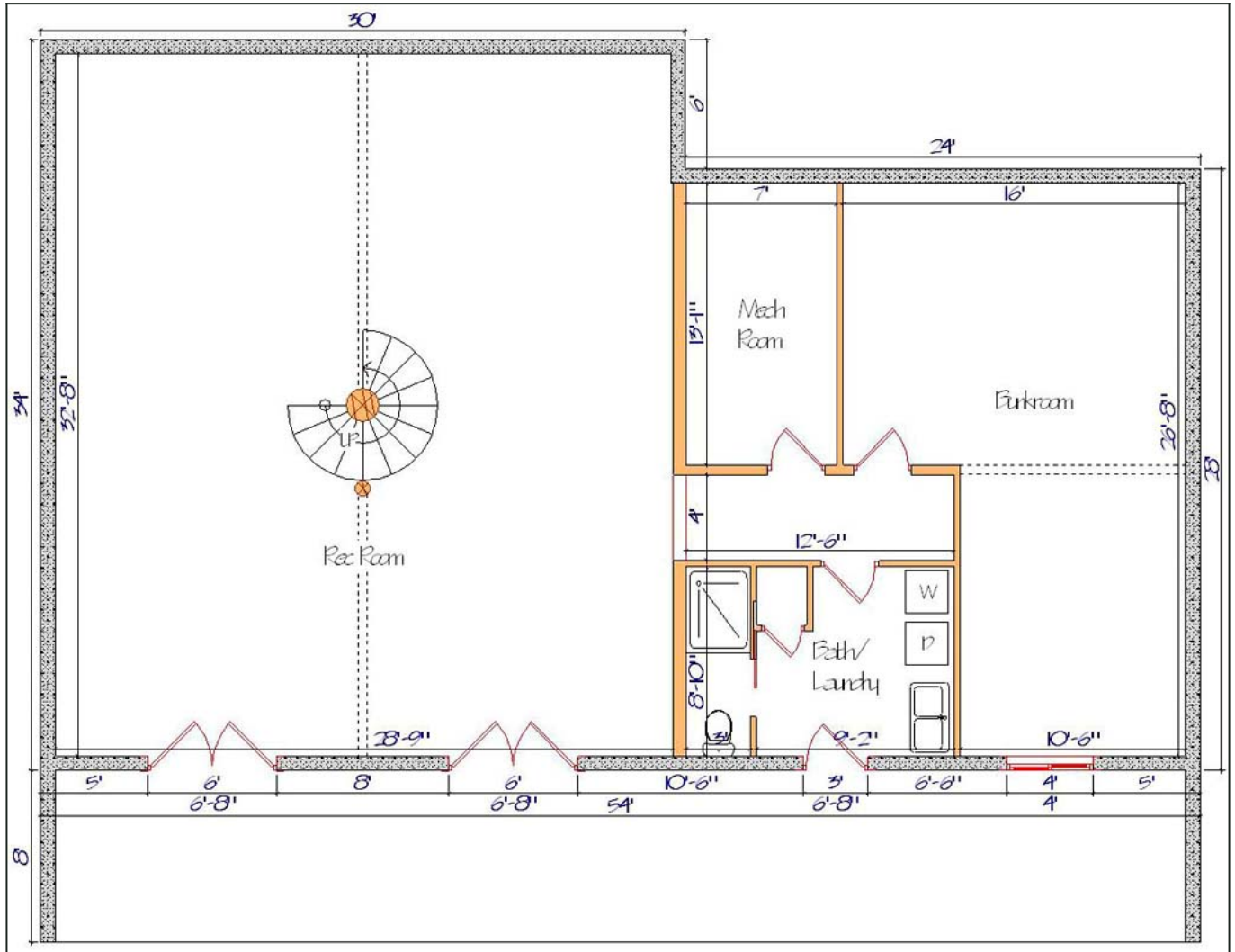
Floor Plan — View 3
