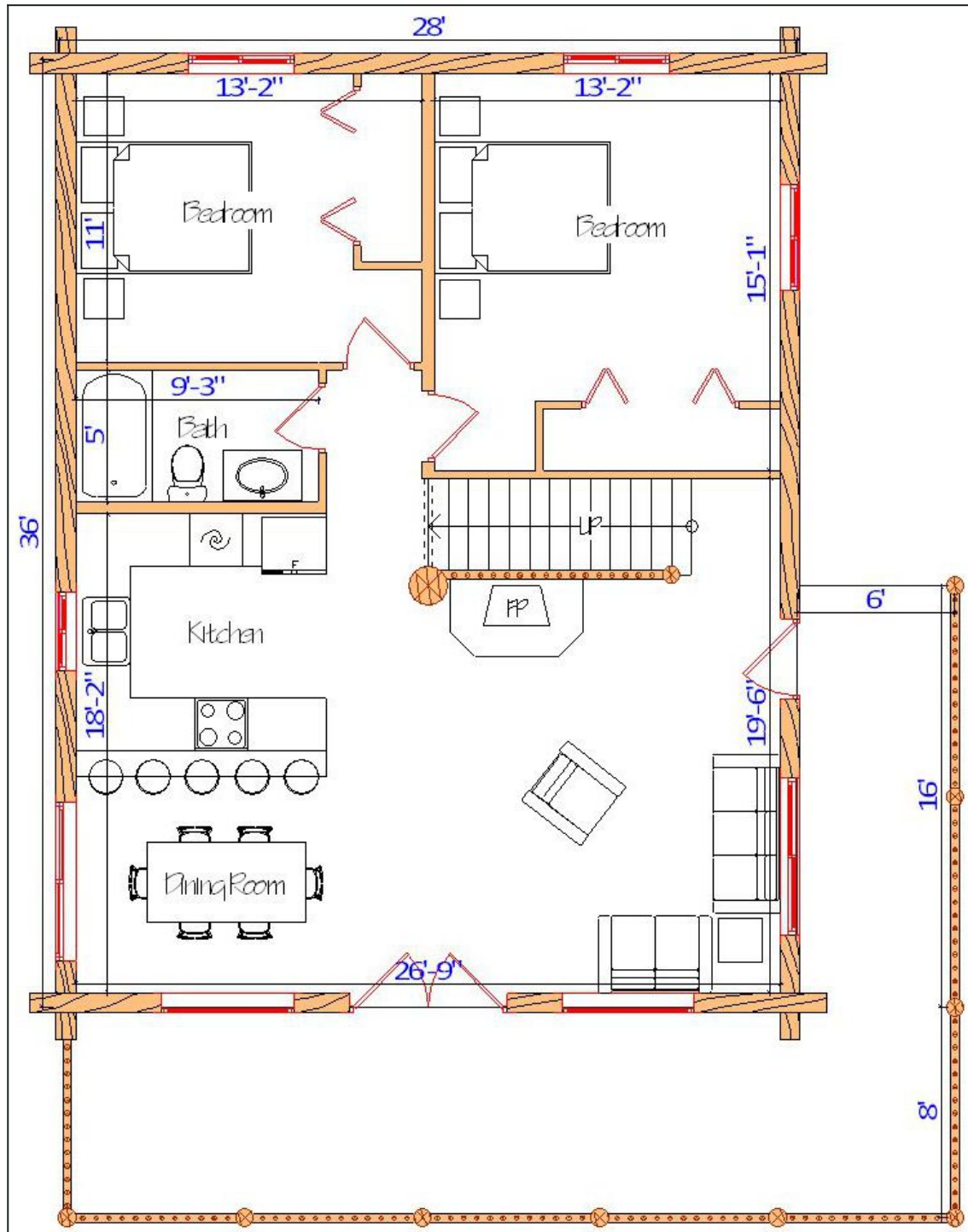
Floor Plan — View 2
