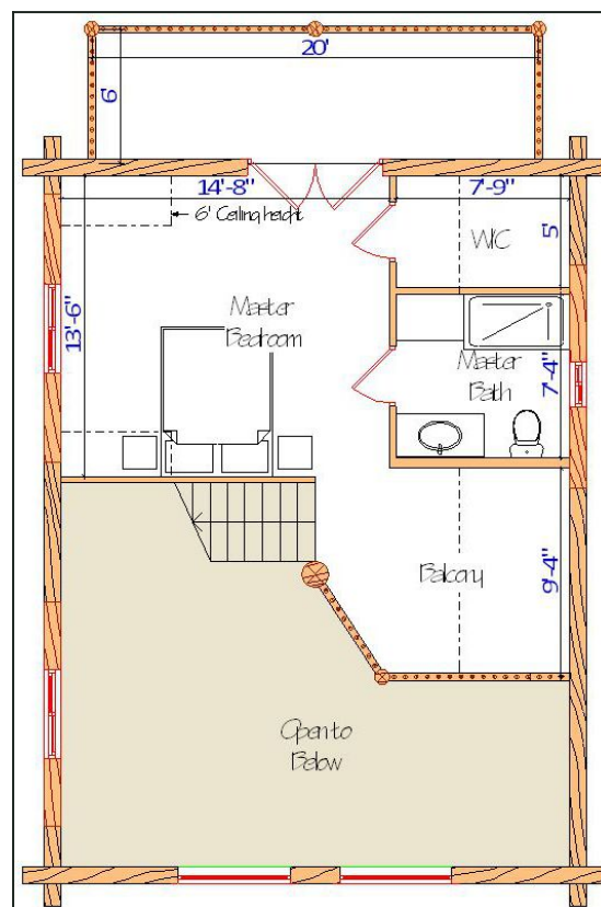
Floor Plan — View 1
