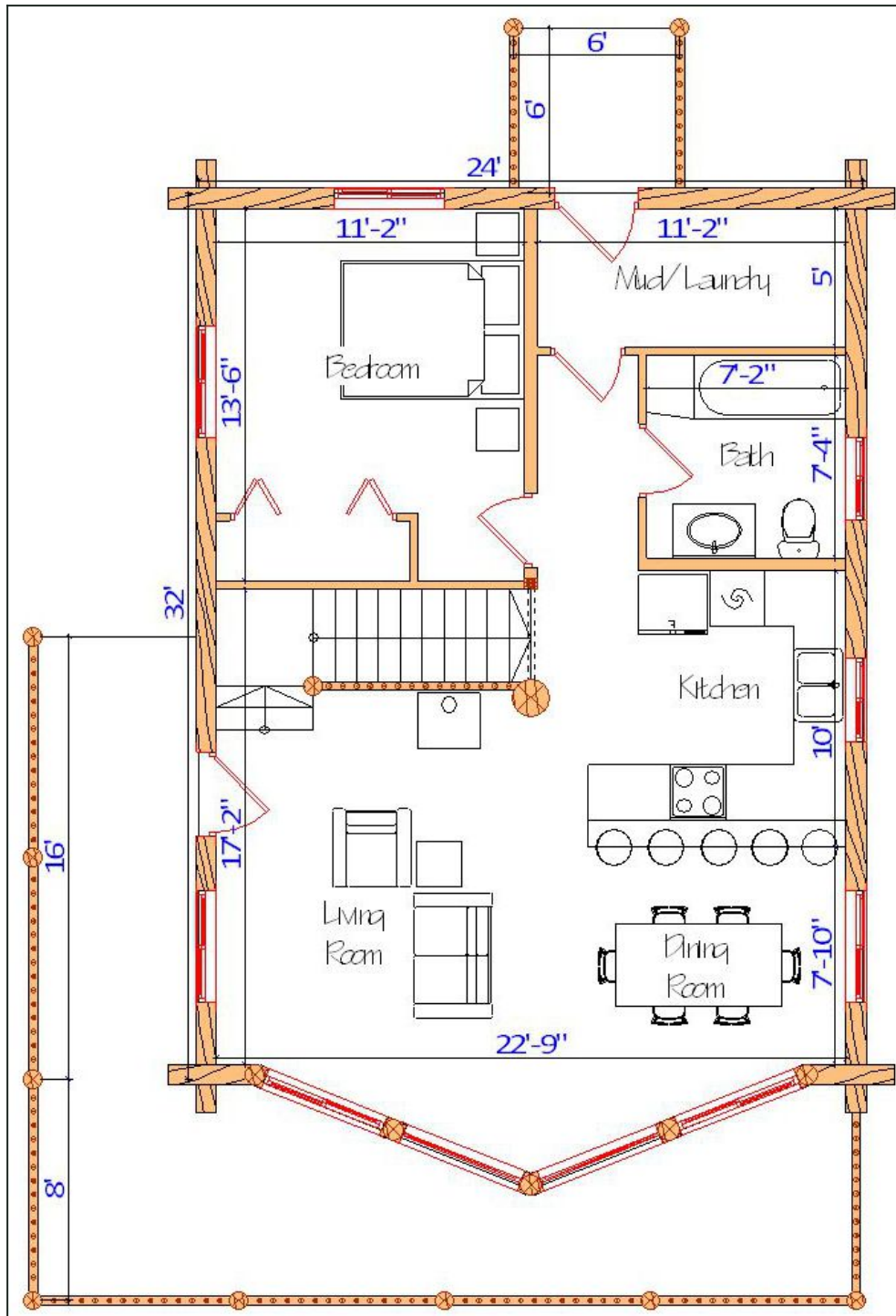
Floor Plan — View 2
