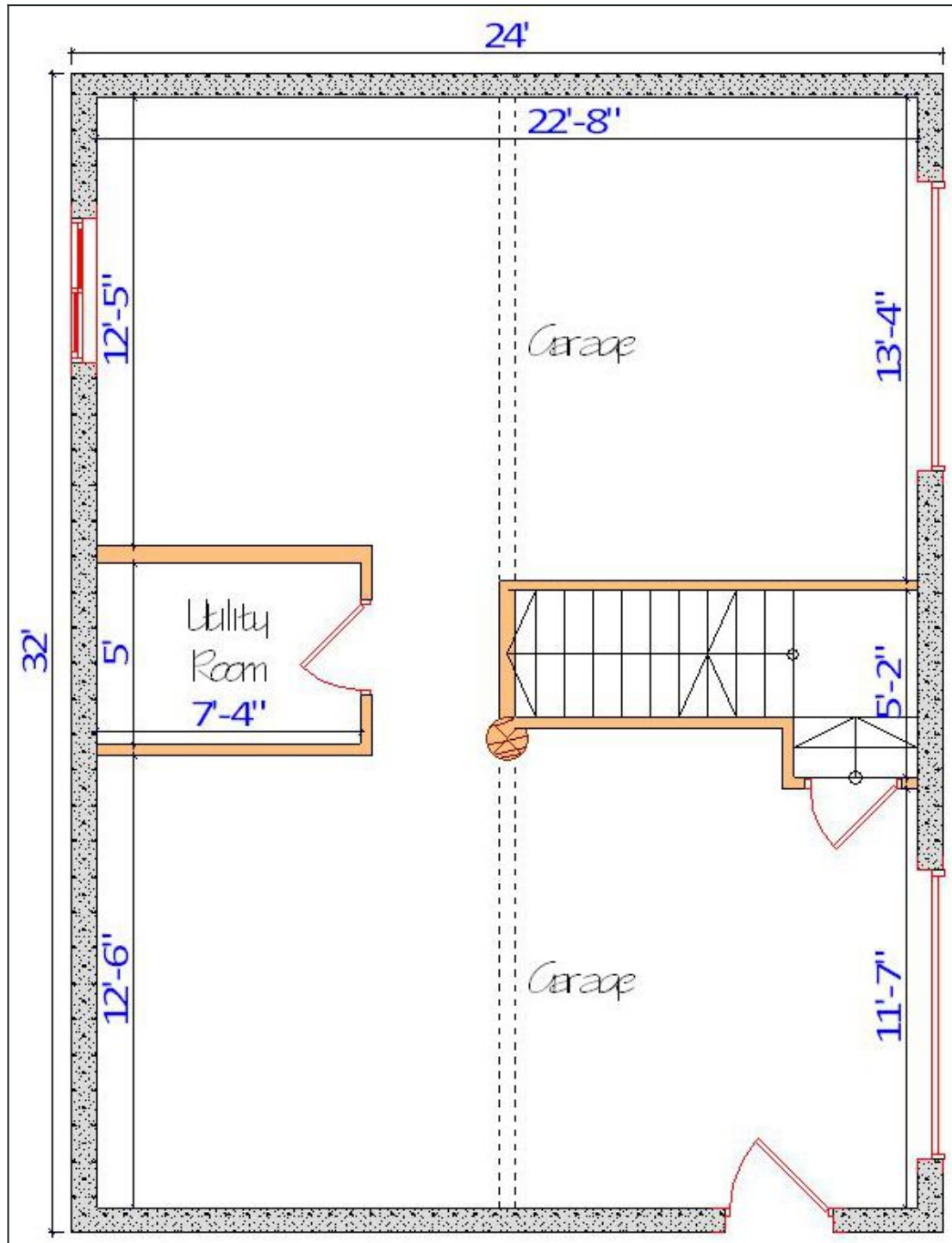
Floor Plan — View 3
