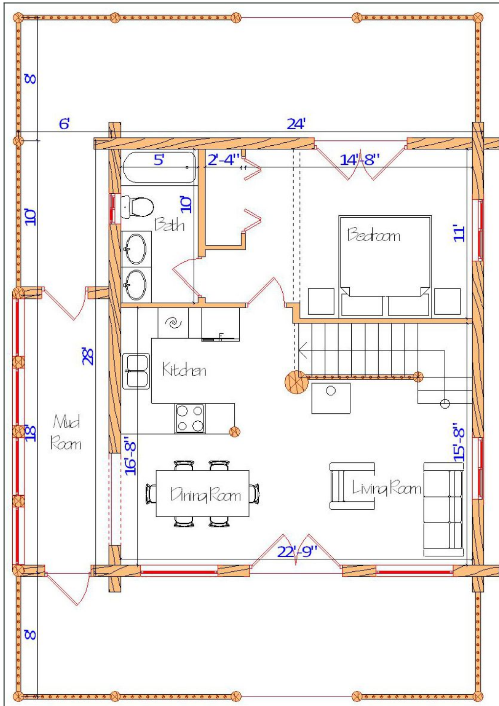
Floor Plan — View 2
