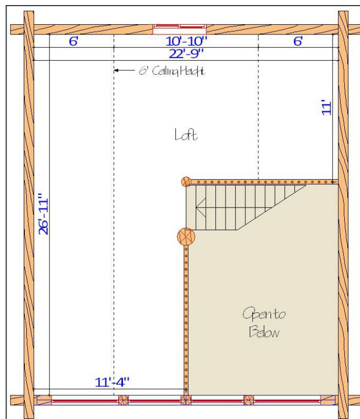
Floor Plan — View 1
