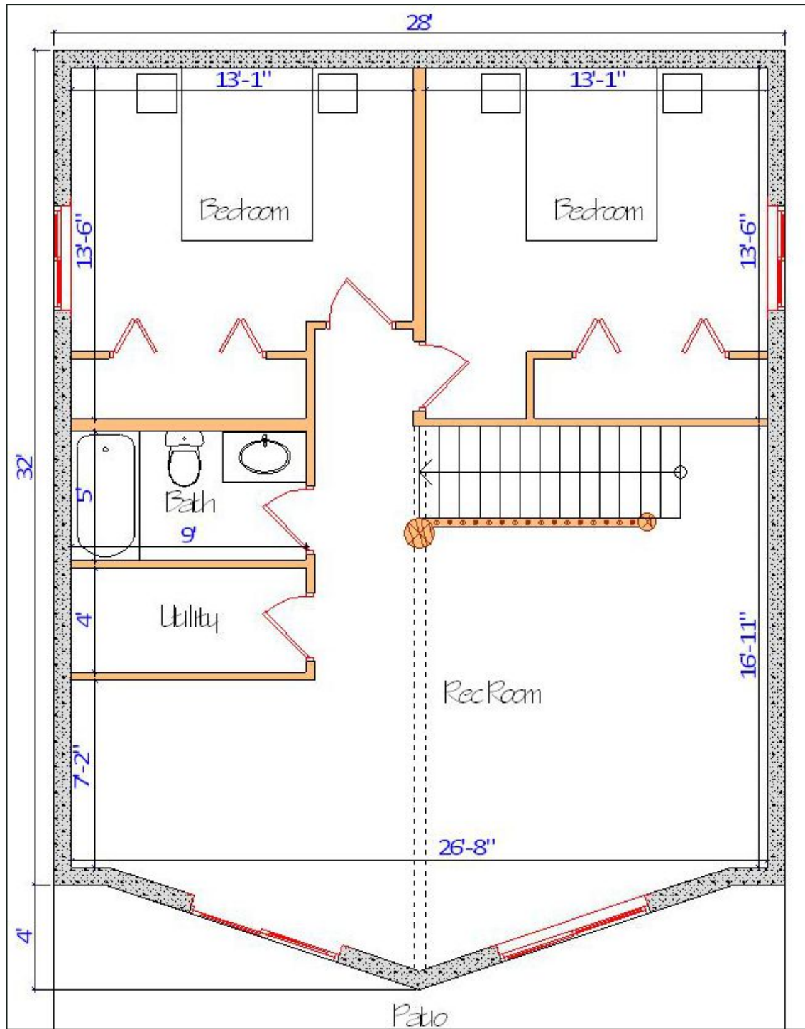
Floor Plan — View 3
