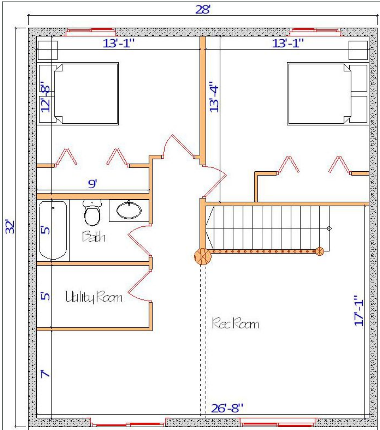
Floor Plan — View 3
