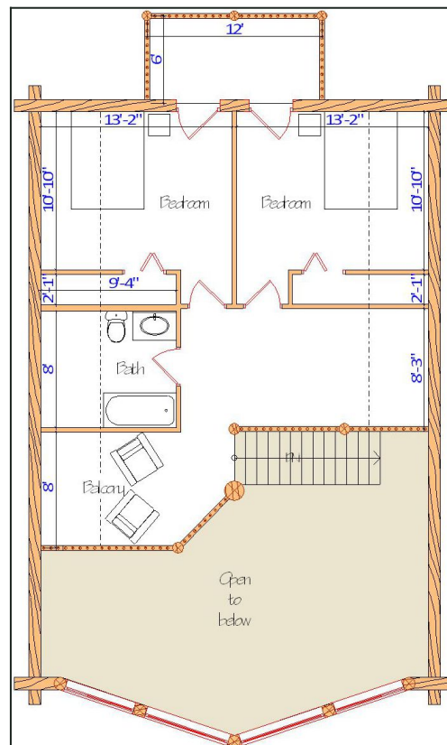
Floor Plan — View 1
