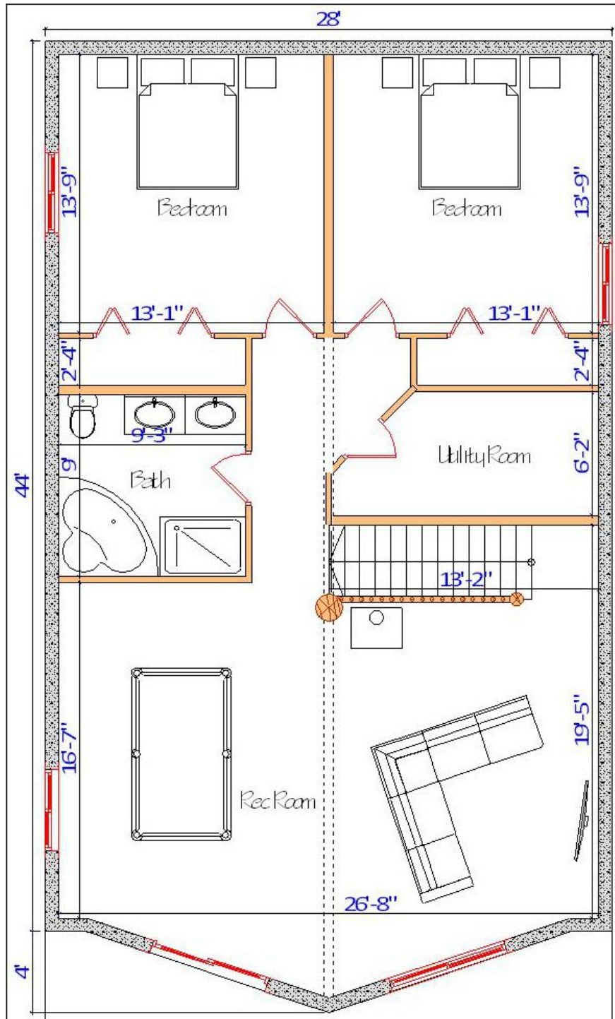
Floor Plan — View 2
