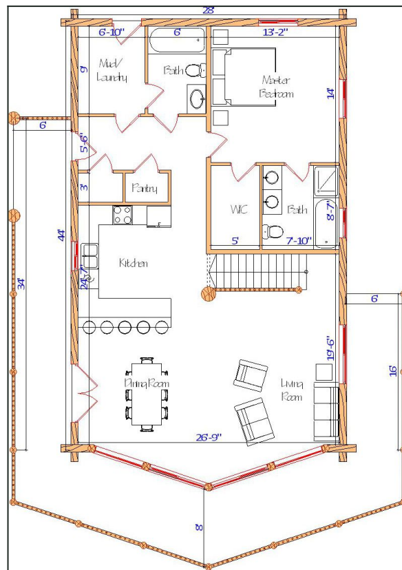
Floor Plan — View 1
