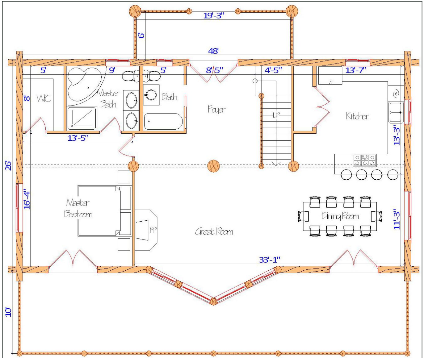
Floor Plan — View 2
