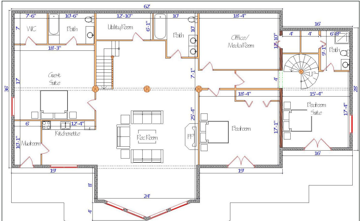
Floor Plan — View 3
