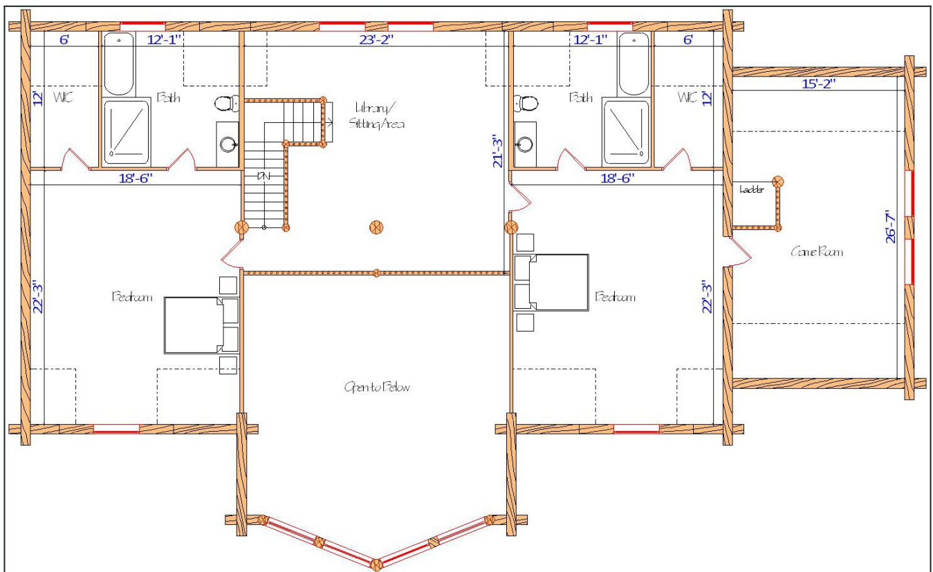
Floor Plan — View 1
