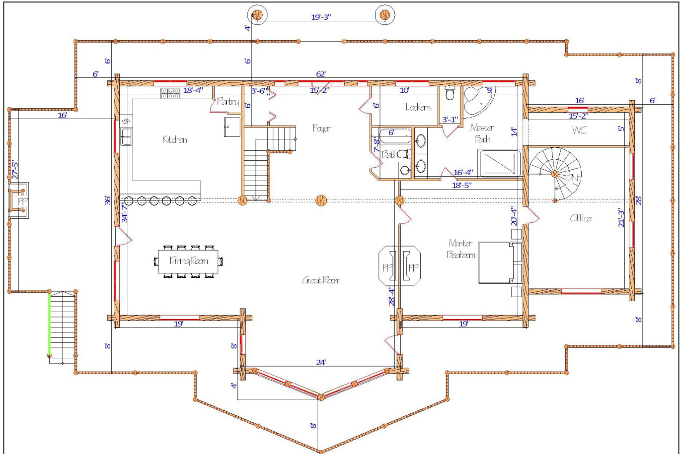
Floor Plan — View 2
