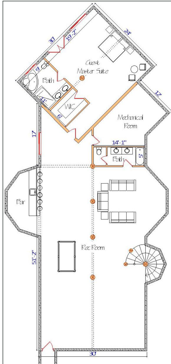
Floor Plan — View 3
