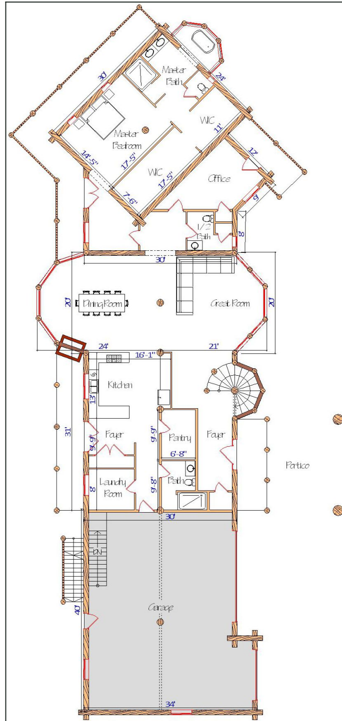
Floor Plan — View 2
