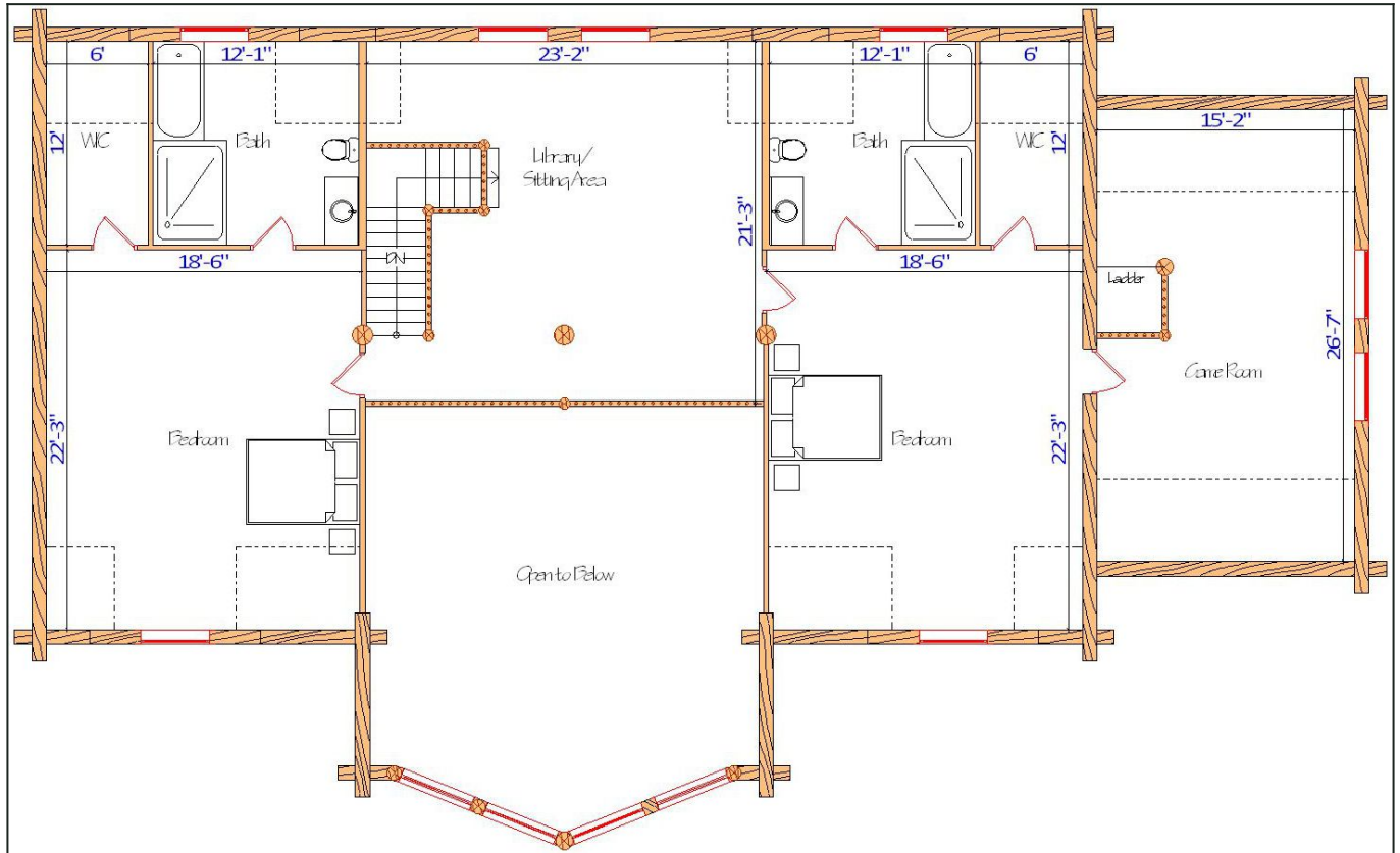
Floor Plan — View 2
