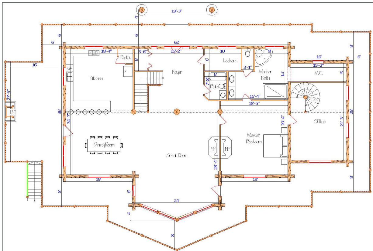
Floor Plan — View 1
