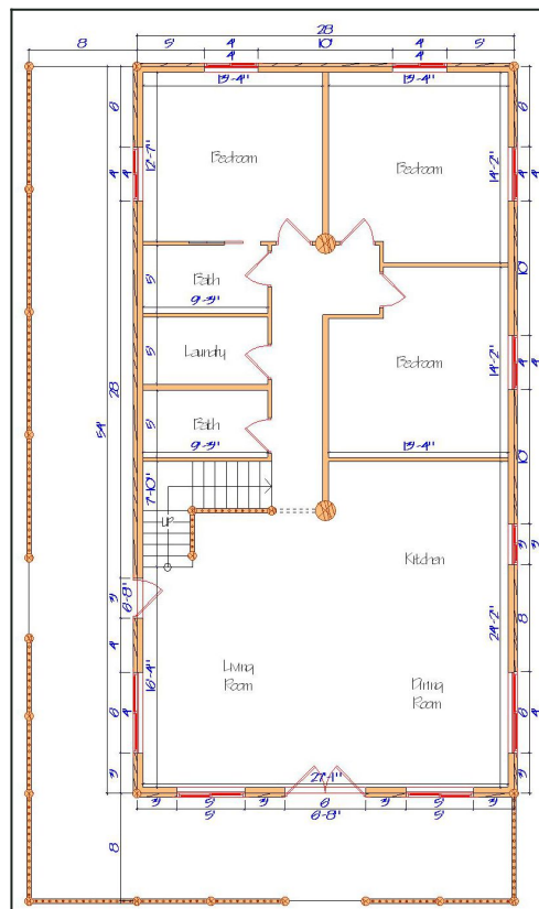
Floor Plan — View 1
