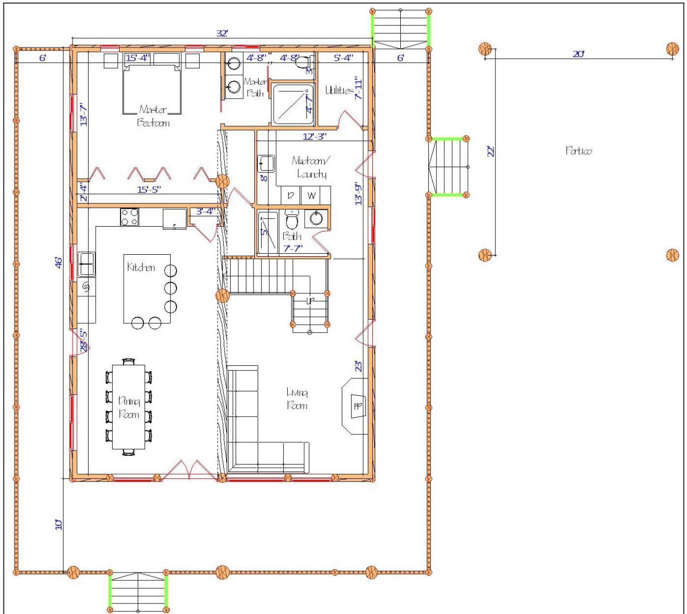
Floor Plan — View 2
