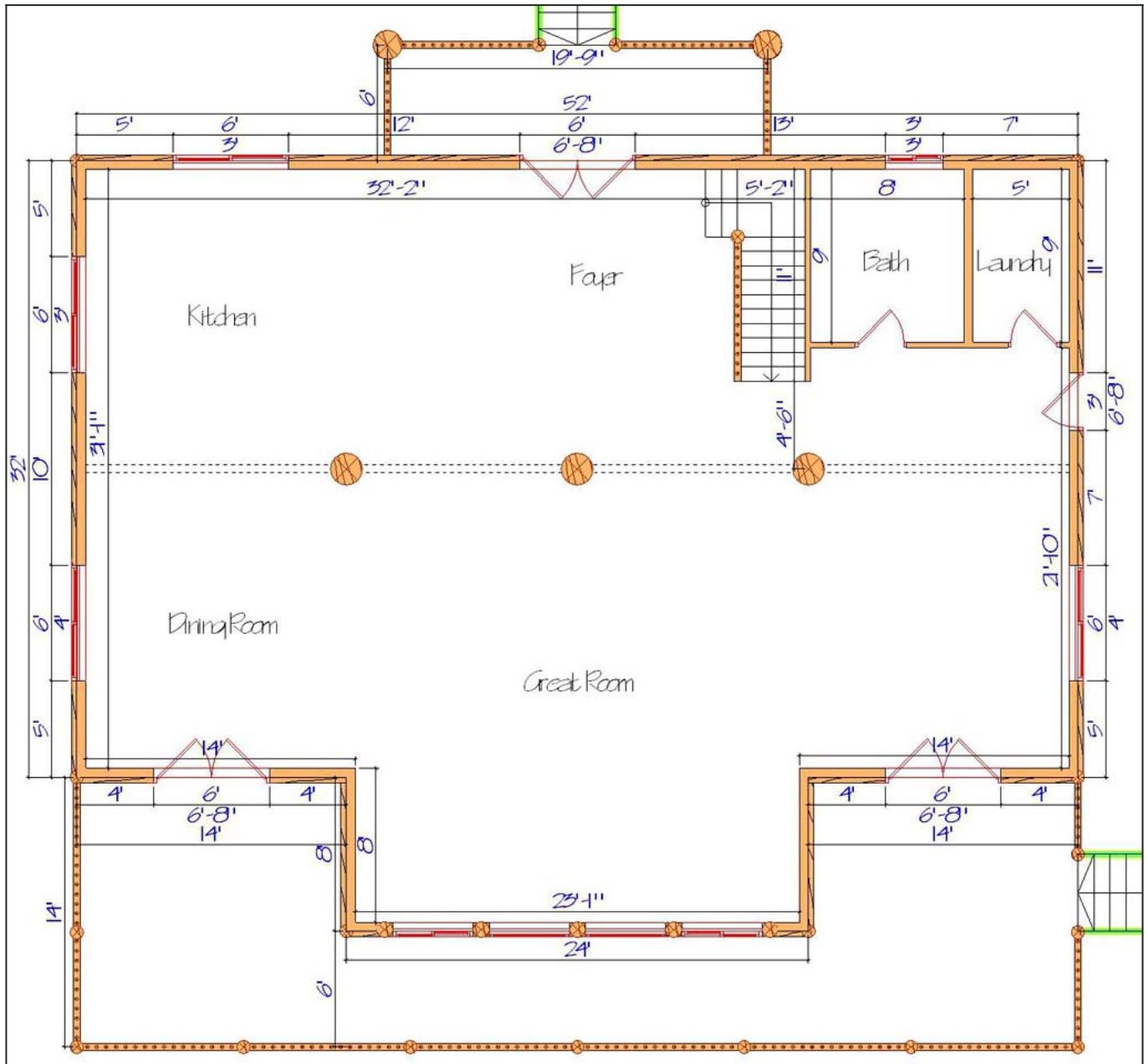
Floor Plan — View 2
