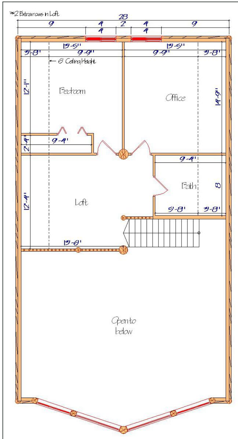
Floor Plan — View 3
