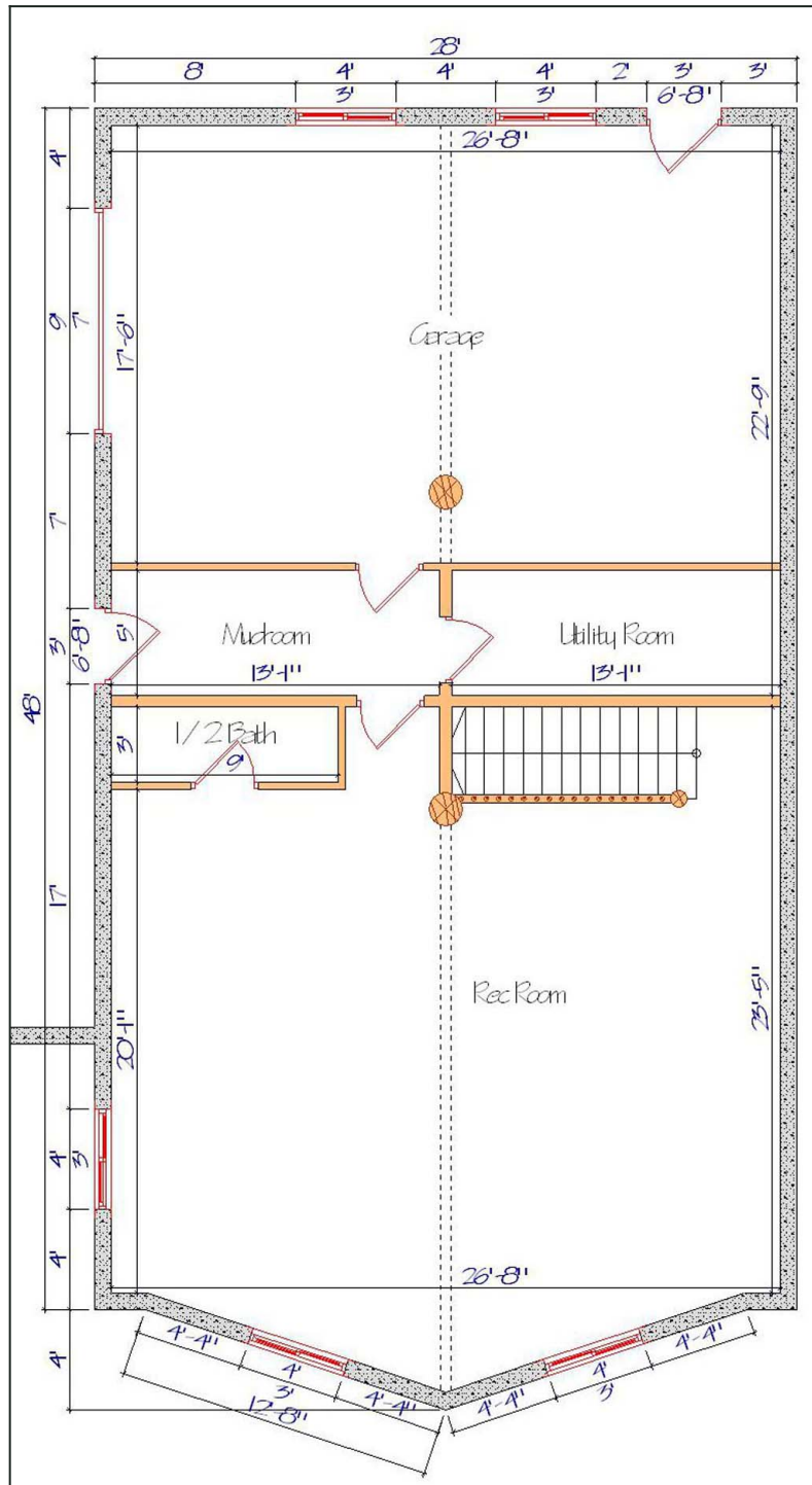
Floor Plan — View 2
