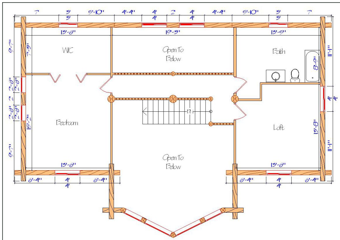
Floor Plan — View 1
