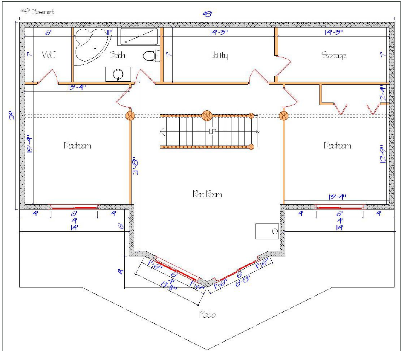
Floor Plan — View 3
