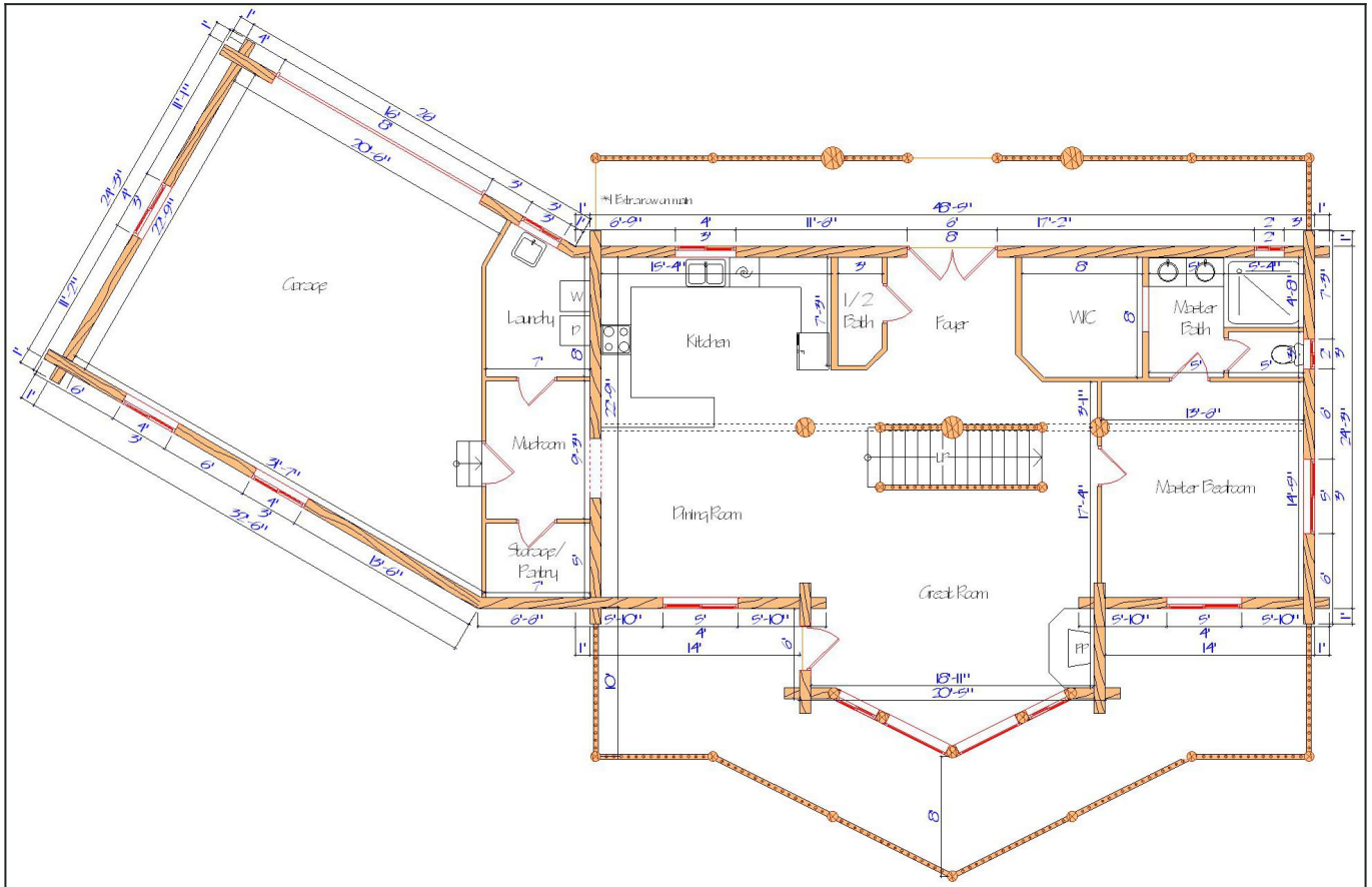
Floor Plan — View 2
