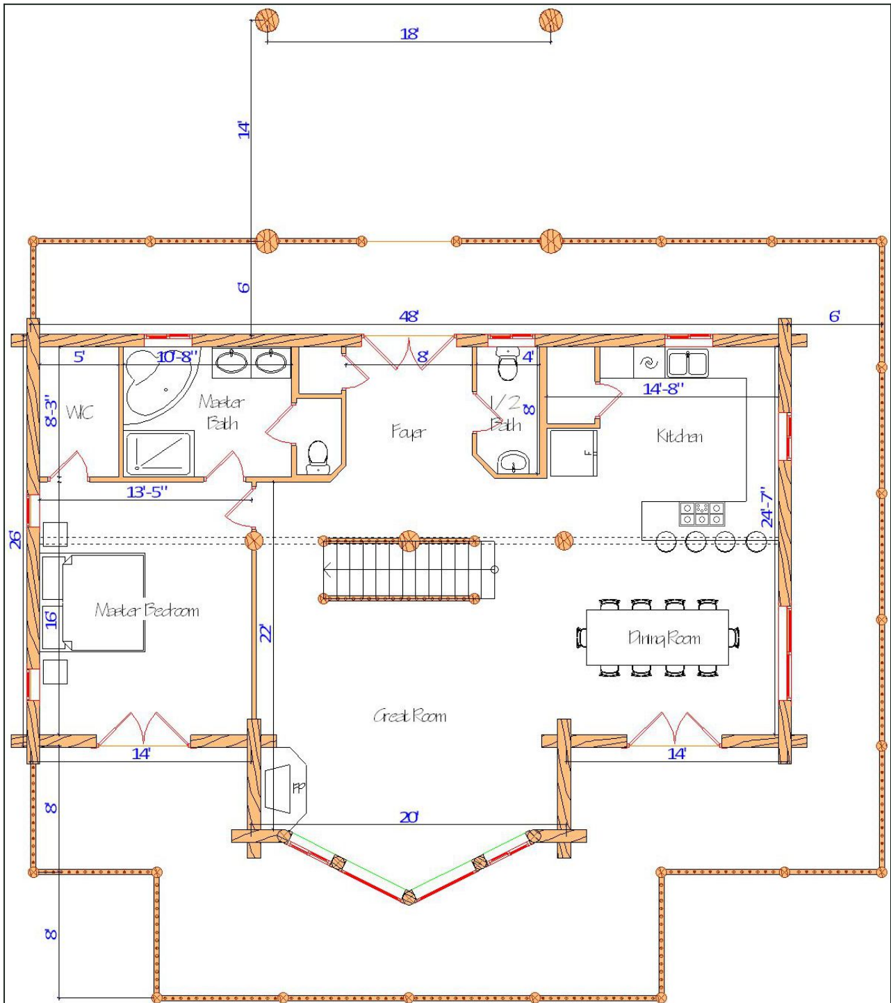
Floor Plan — View 2
