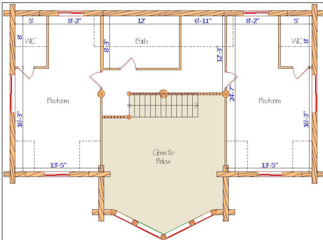
Floor Plan — View 1
