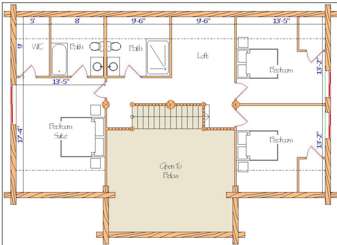
Floor Plan — View 1
