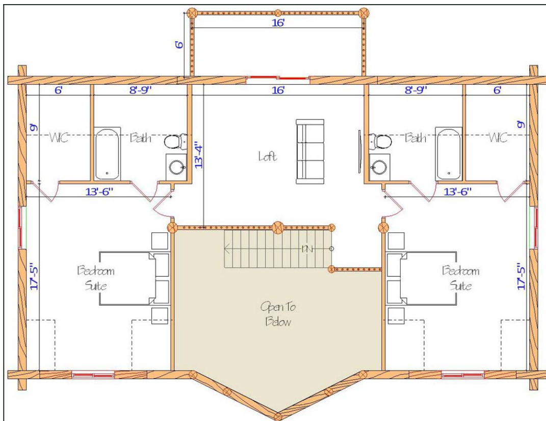
Floor Plan — View 1
