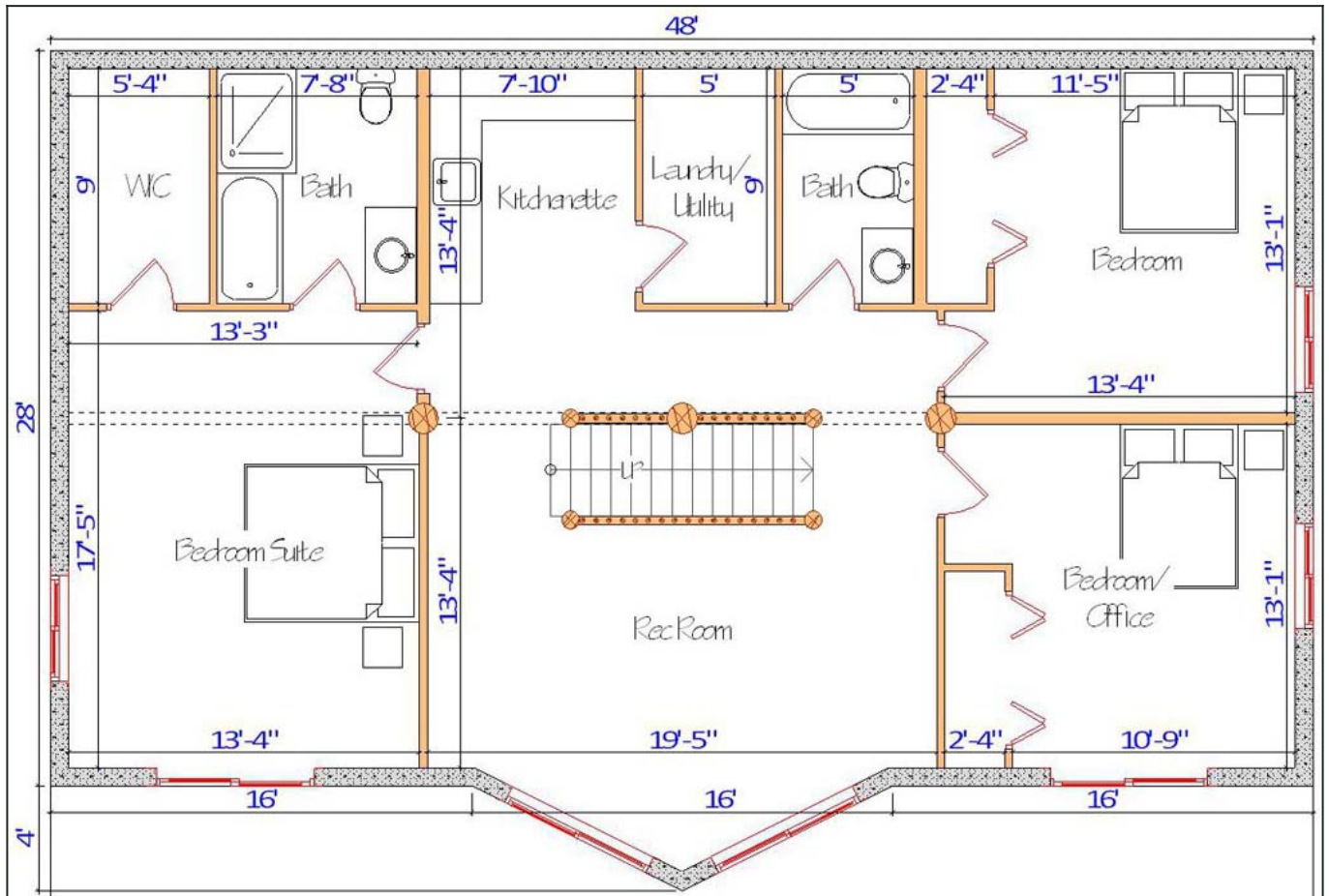
Floor Plan — View 3
