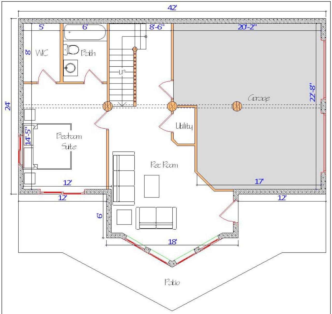
Floor Plan — View 3
