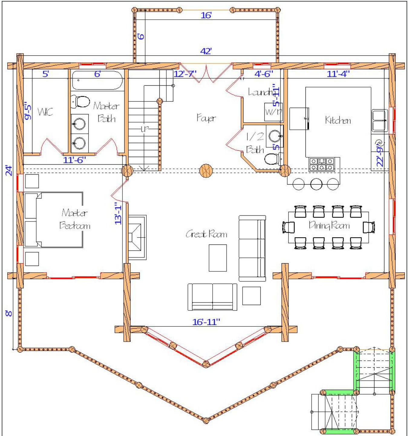
Floor Plan — View 2
