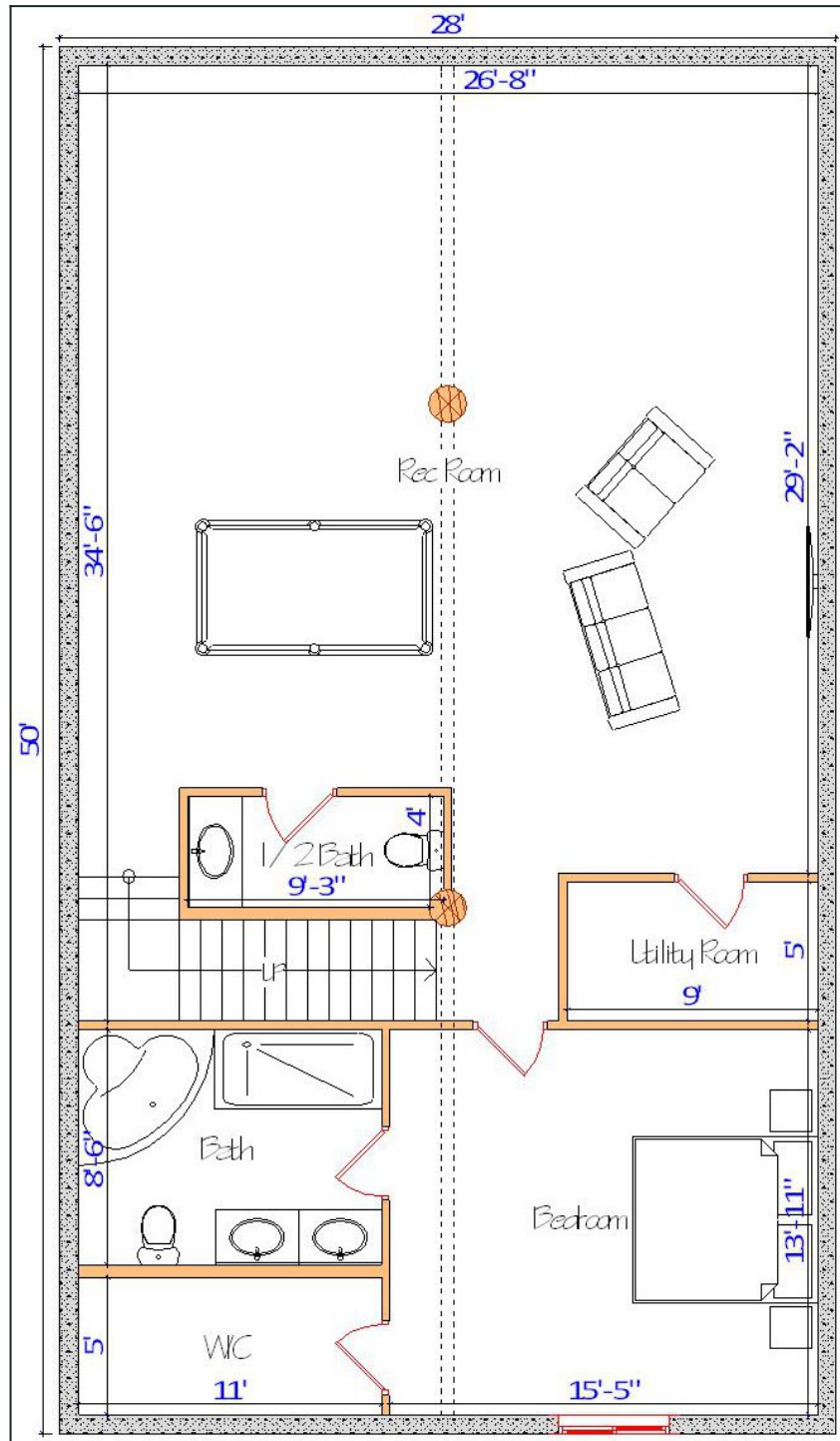
Floor Plan — View 2
