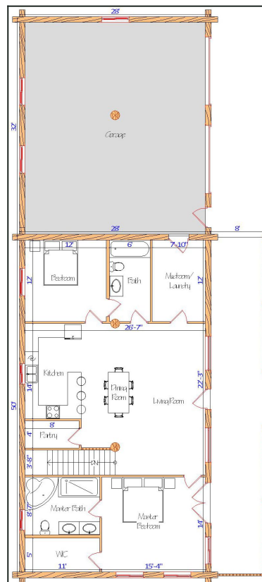
Floor Plan — View 1
