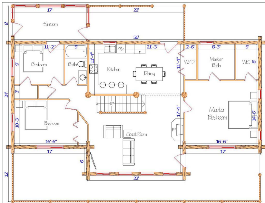
Floor Plan — View 1
