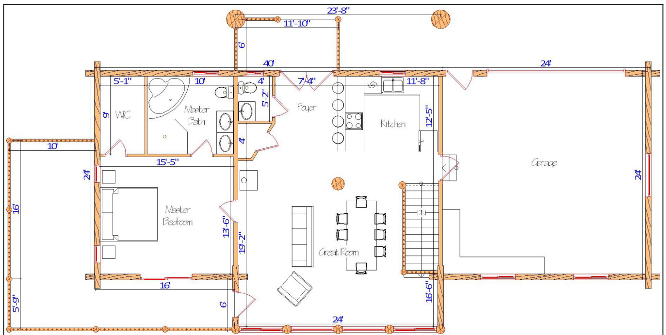
Floor Plan — View 1
