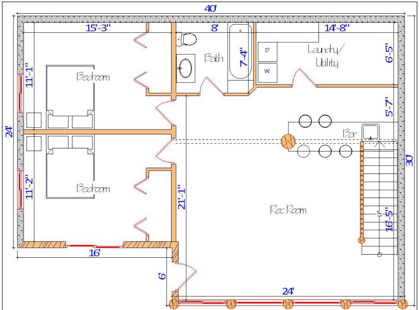
Floor Plan — View 2
