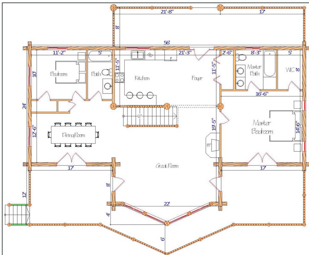
Floor Plan — View 1
