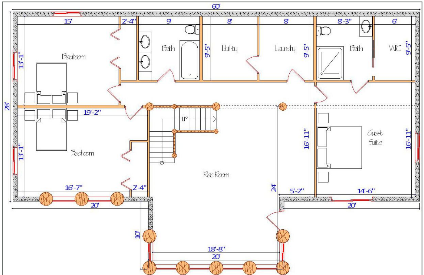
Floor Plan — View 3
