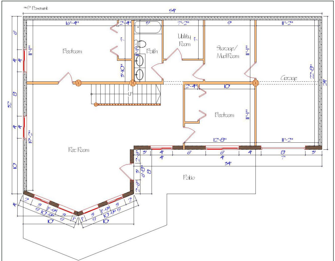
Floor Plan — View 2
