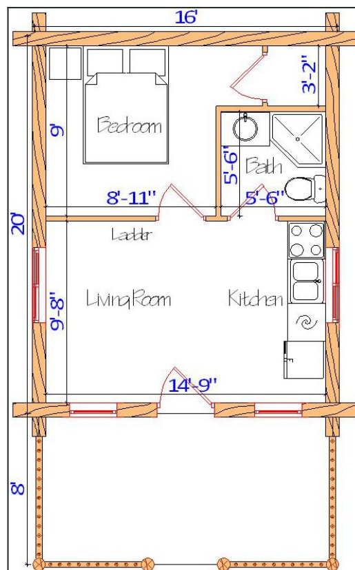
Floor Plan — View 1
