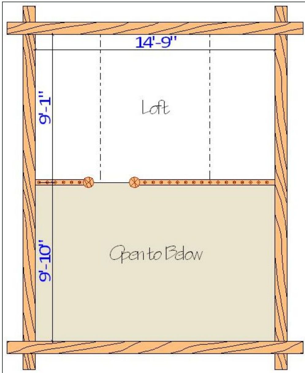
Floor Plan — View 2
