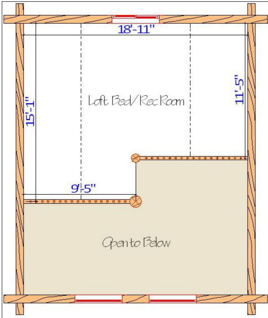
Floor Plan — View 2
