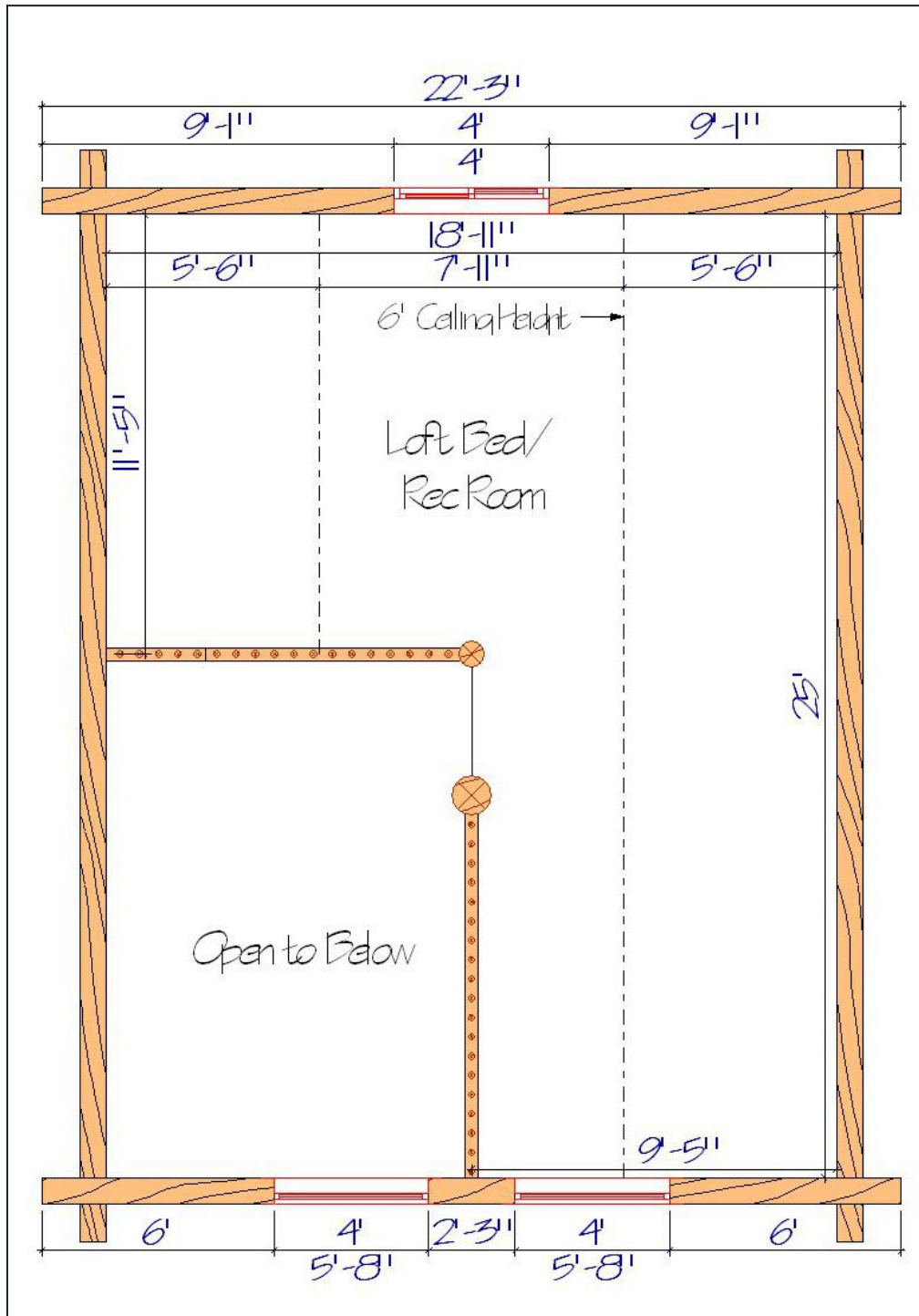
Floor Plan — View 2
