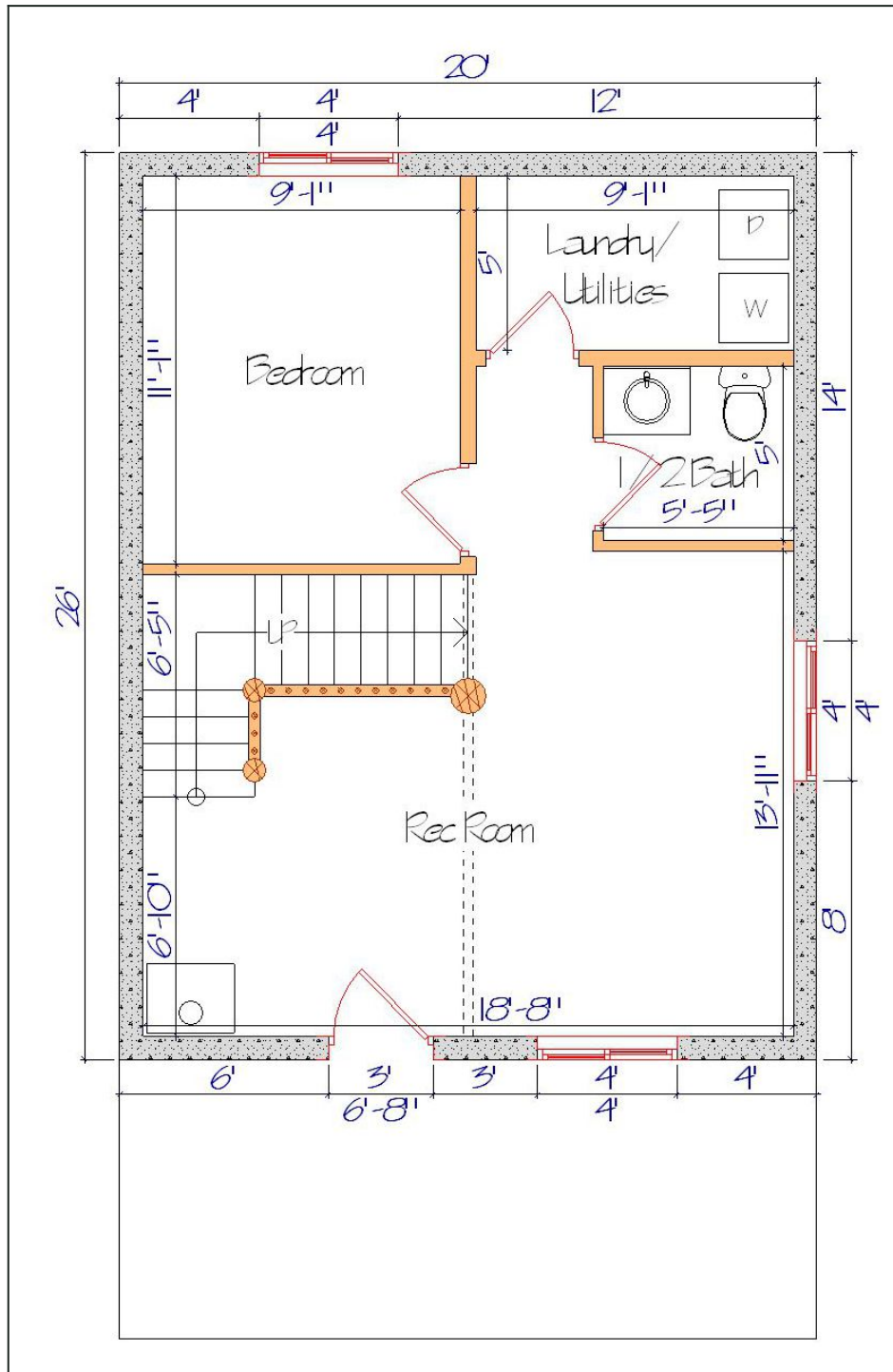
Floor Plan — View 3
